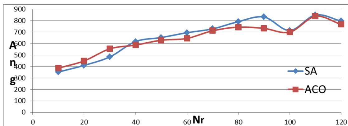
Fig. 6.4. Dependence of total rotation angle of the number of robots for 300 targets.
