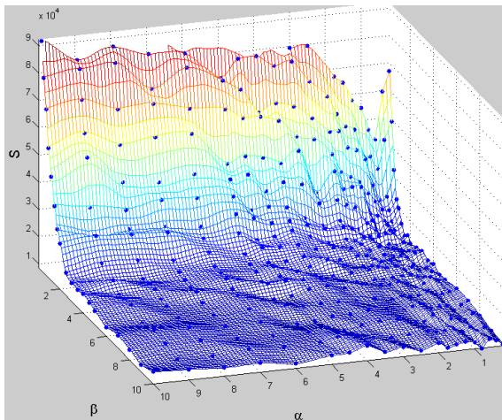
Fig.4. Dependence of total path length of the algorithm parameters: S=S(\alpha, \beta) .
