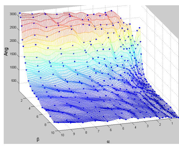
Fig.5. Dependence of total rotation angle of the algorithm parameters: Ang=Ang(\alpha, \beta) .
